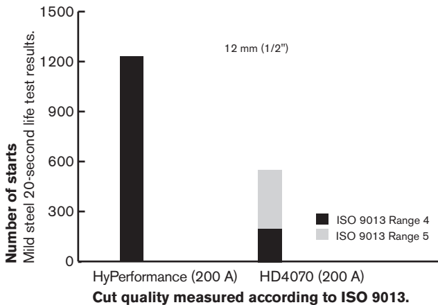
Cut quality measured according to ISO 9013.
